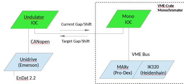
Figure 1: Interfaces used for CM from monochromator to motion controller (VME-Bus), encoder card (VME-Bus) and undulator IOC (CAN). VME based hardware for monochromator: MVME162 (Motorola), MAXv (Pro-Dex), or VME6, OMS58 (OMS), IK320 (Heidenhain).
