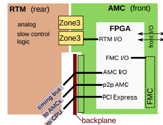
Figure 1: MTCA.4 front and rear modules
