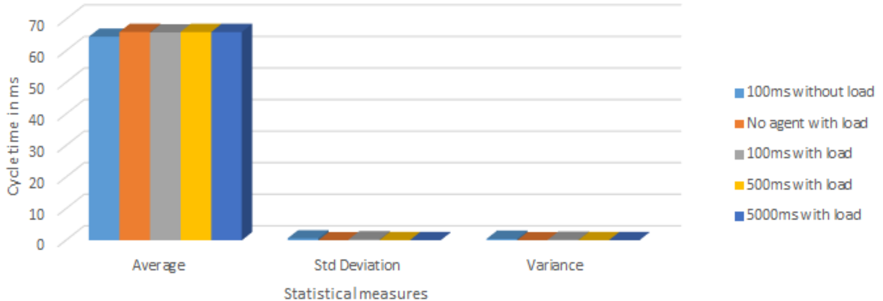
Impact of Diagnostics Monitoring on a SIEMENS PLC S7-414-2
